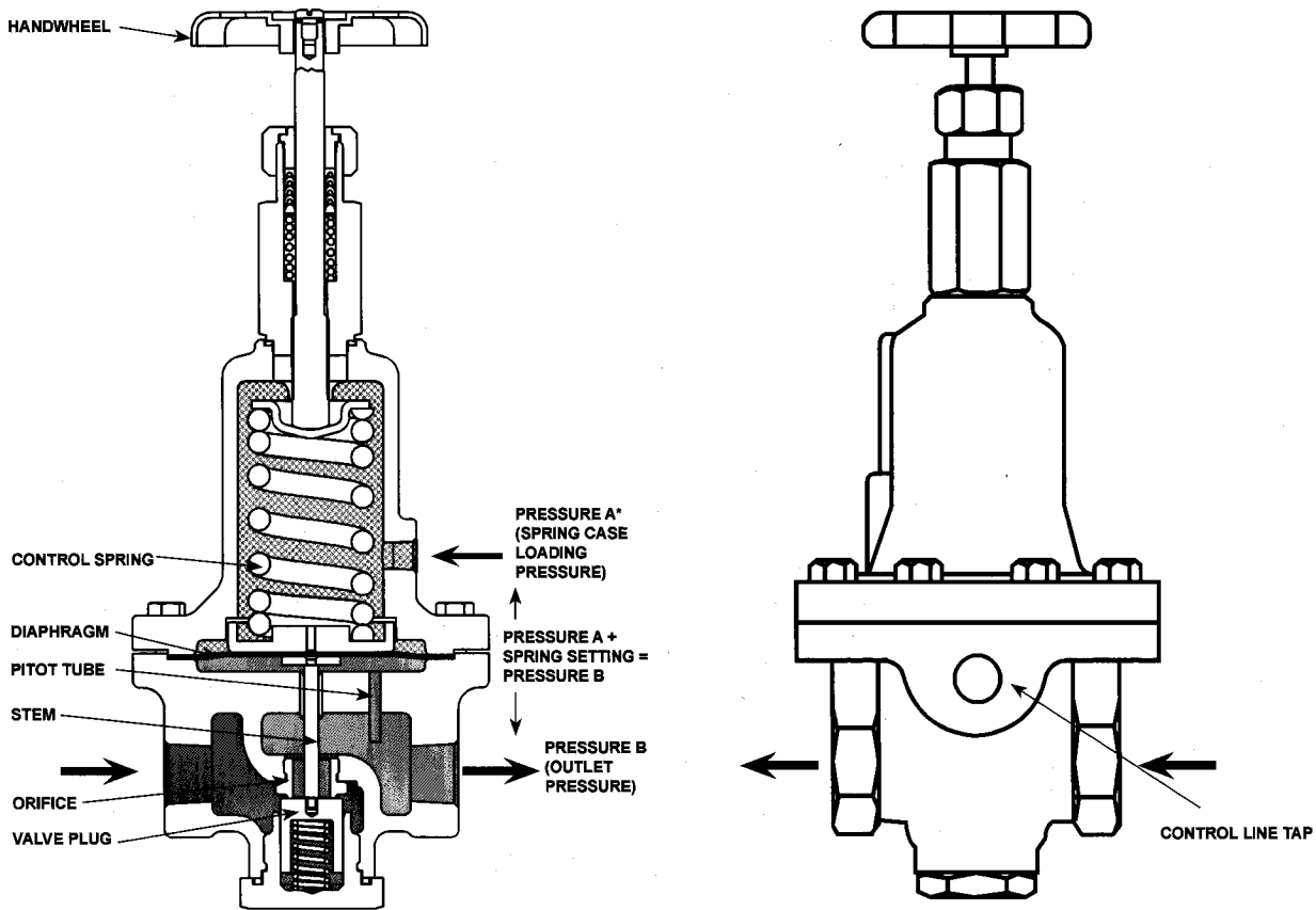
FRONT AND INTERNAL VIEW OF TYPES MR95HD AND MR95HDP WITH INTERNAL PRESSURE REGISTRATION
