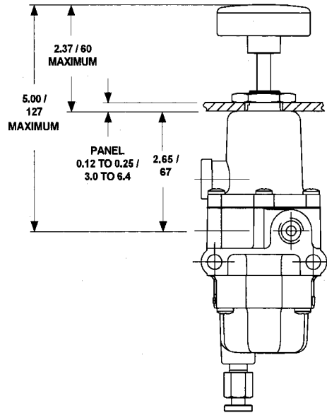
DIMENSIONS FOR PANEL MOUNT OPTION WITH HANDWHEEL
