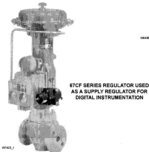
Figure 1. 67C Series Instrument Supply Regulators
