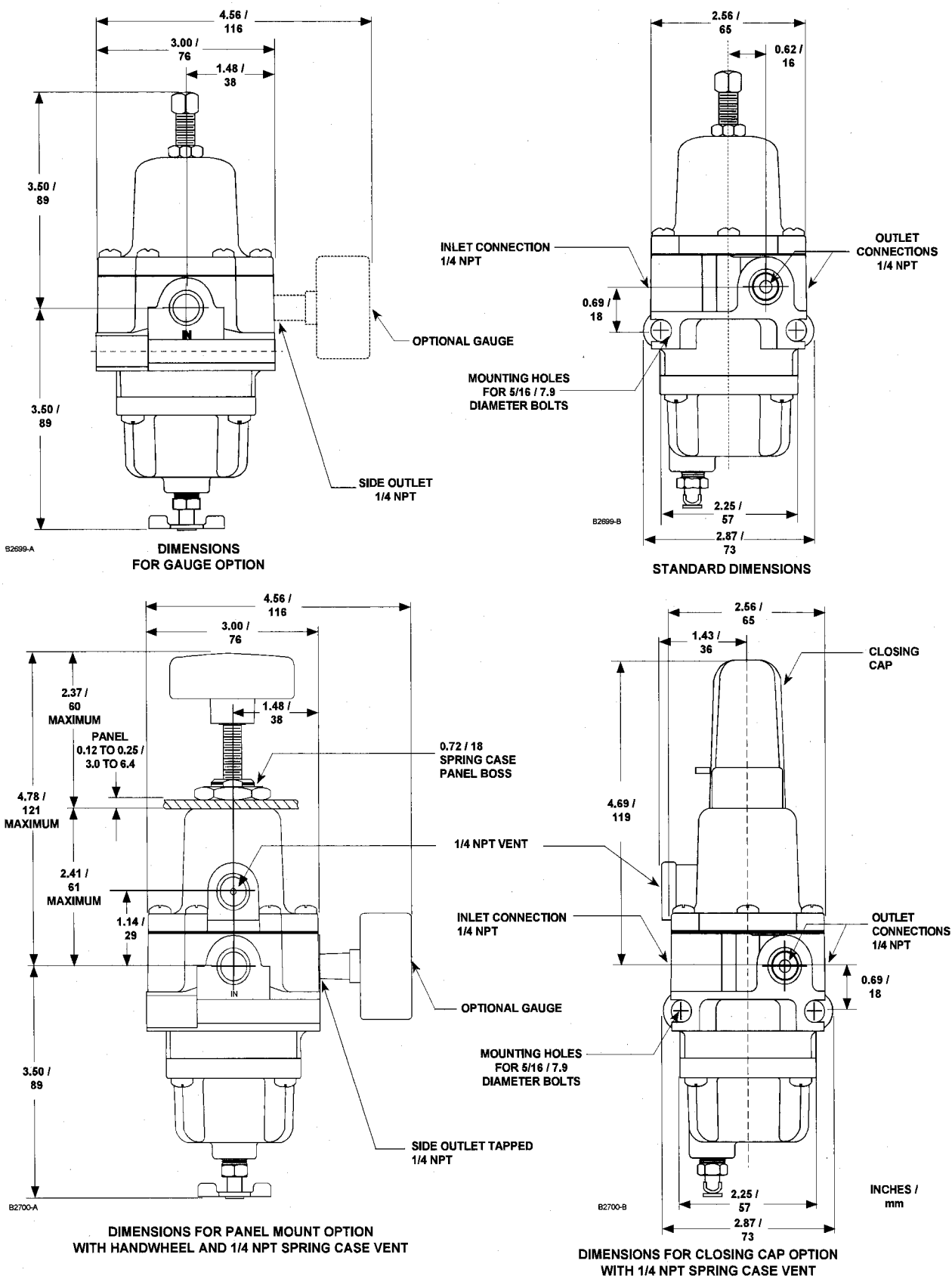
Figure 6. Types 67CF and 67CFR Dimensions
