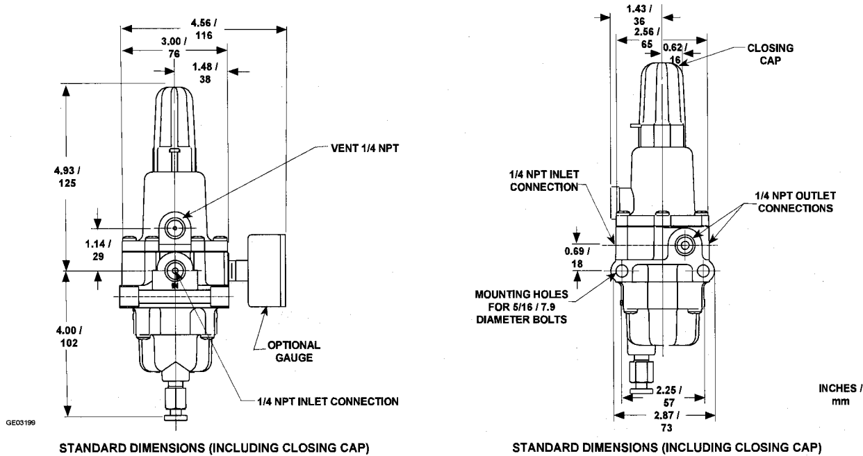
Figure 9. Types 67CFS and 67CFSR Dimensions
