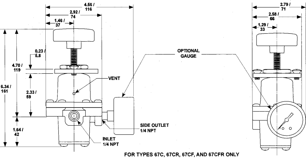
Figure 7. Dimensions for 3-Hole Panel Mount Option With Handwheel and 1/4 NPT Spring Case Vent
