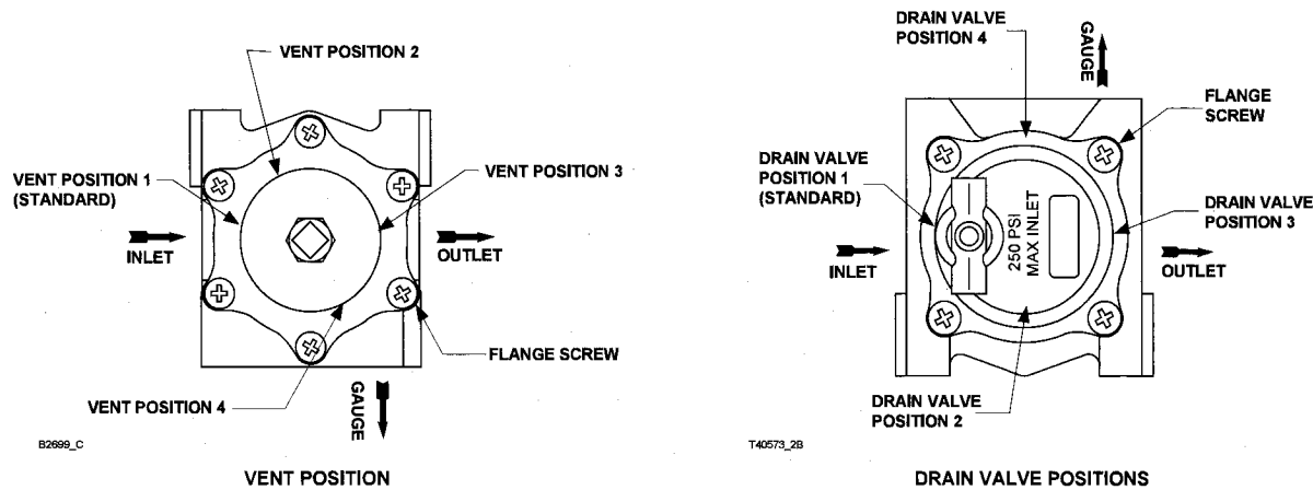
Figure 4. 67C Series Vent and Drain Valve Positions
