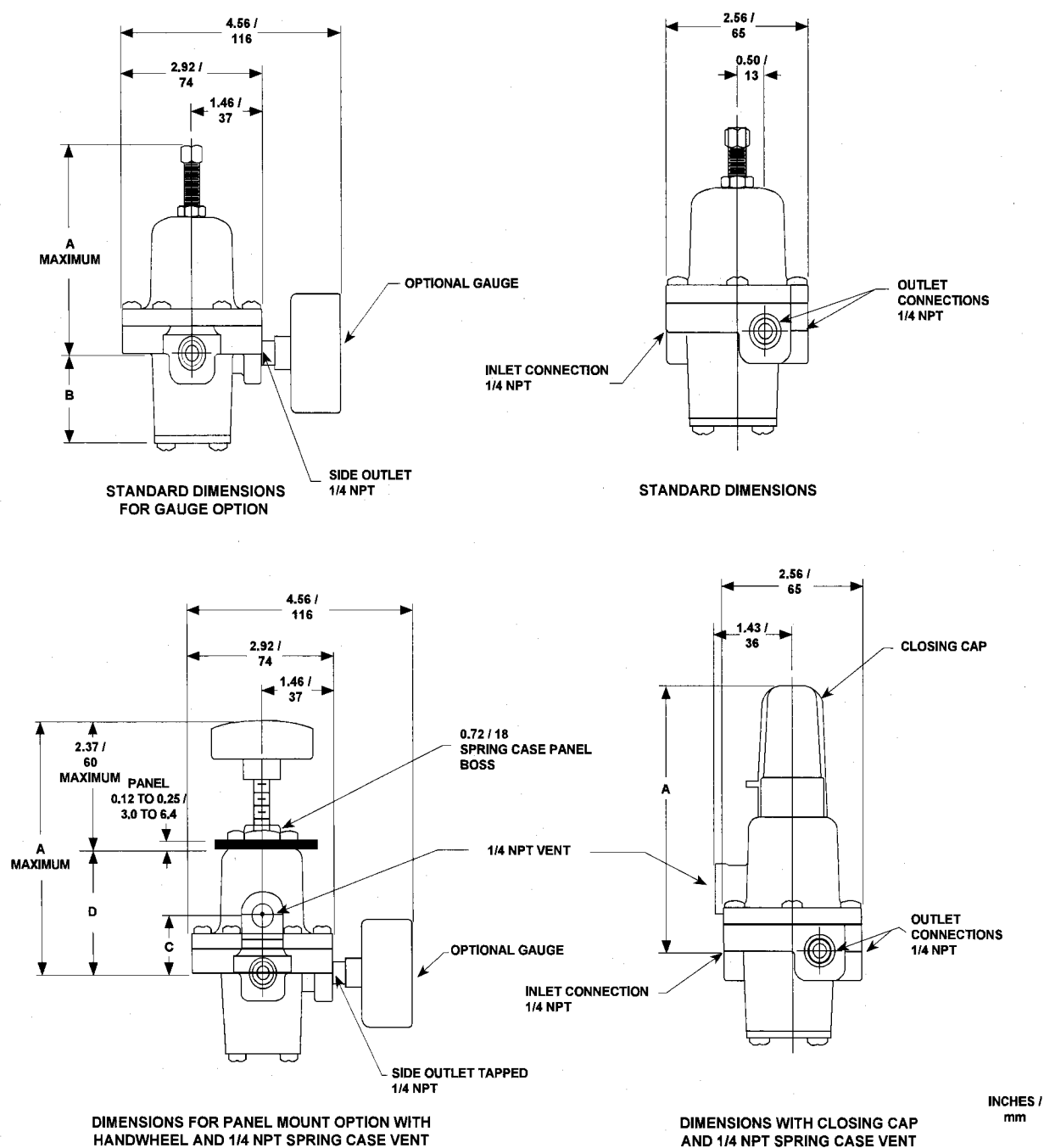
Figure 5. Types 67C, 67CR, 67CS, and 67CSR Dimensions
