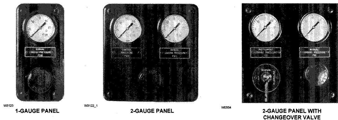
Figure 3. 670 Series Typical Panel Layouts
