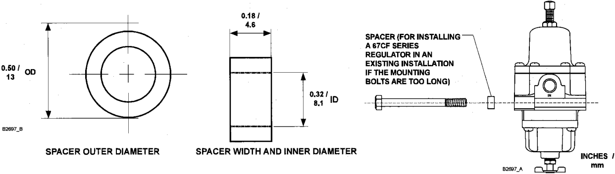
Figure 8. Spacer Dimensions and Installation Schematic
