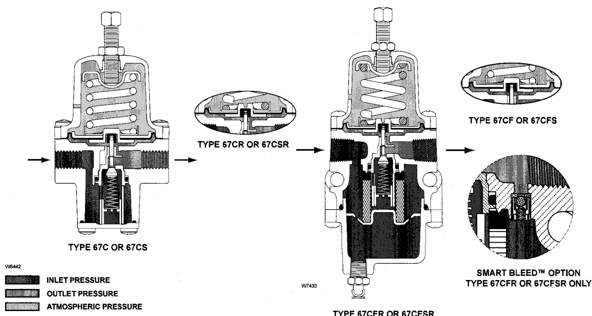
Figure 2. 67C Series Operational Schematics
