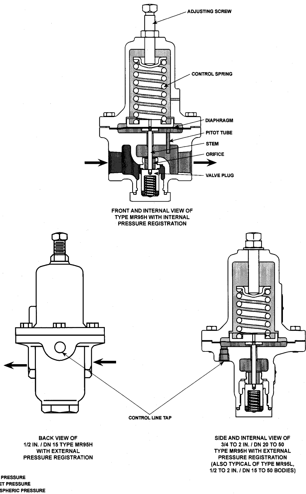
Figure 2. MR95 Series Operational Schematics
