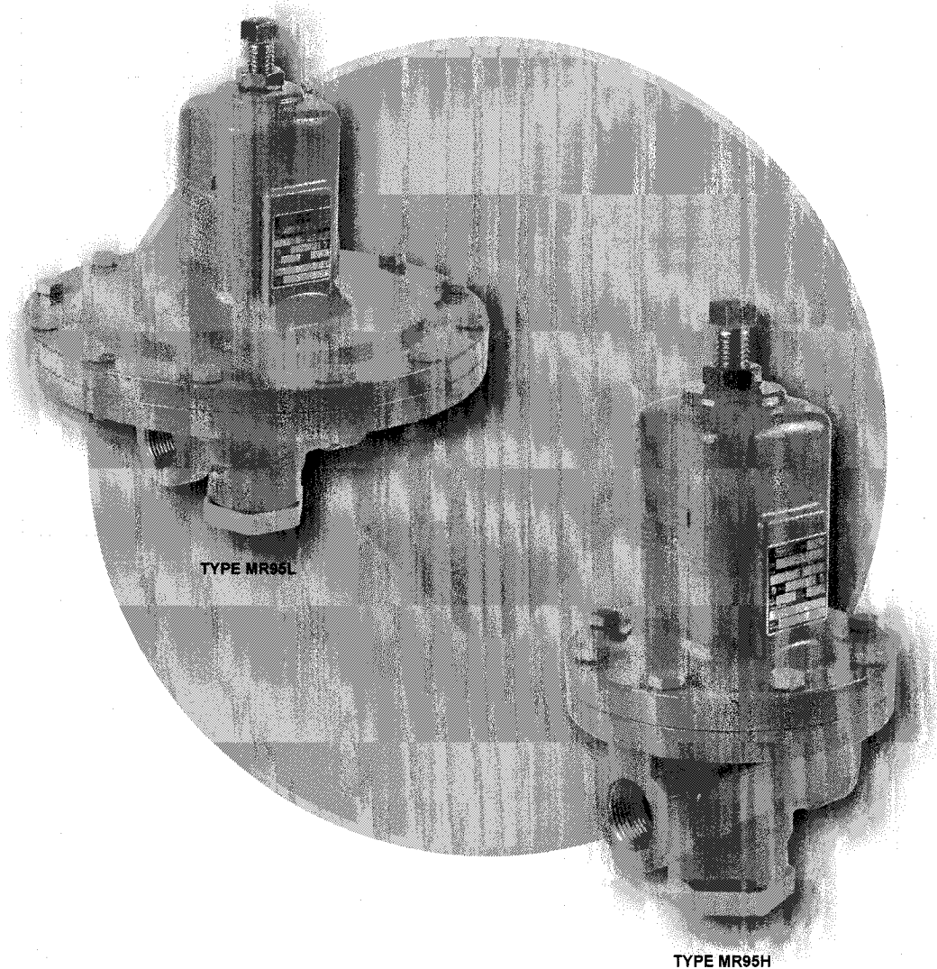
PRESSURE REDUCING REGULATORS
