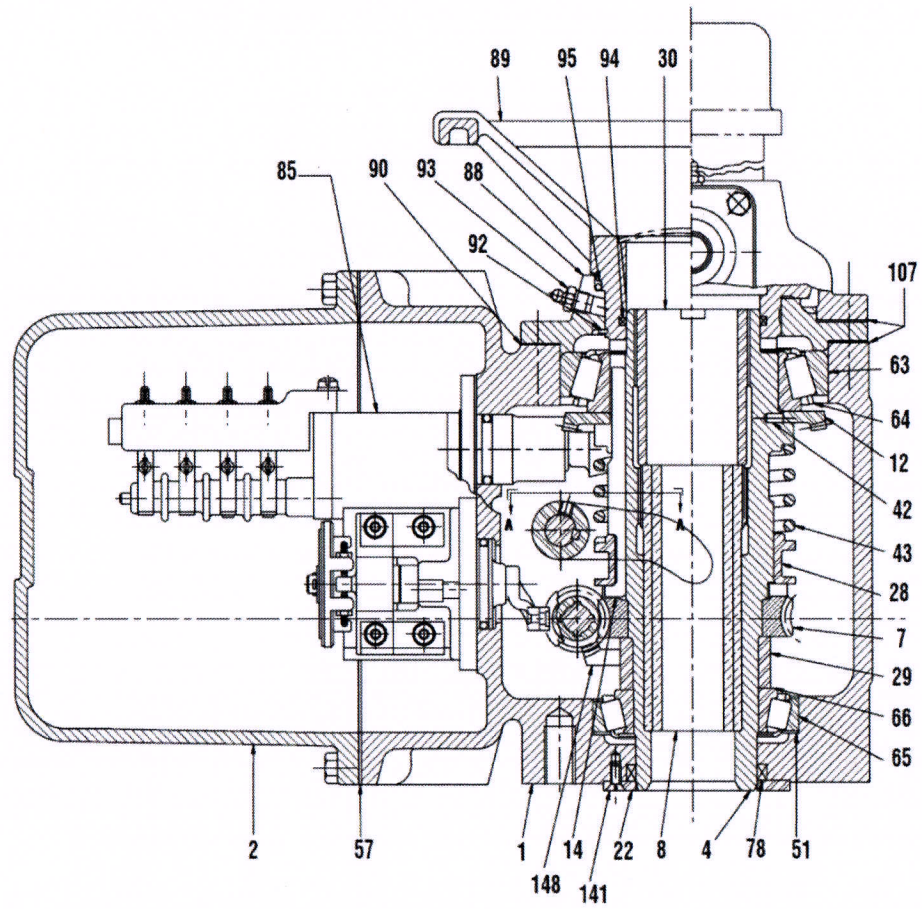
Figure 7.6 – SMB-00 Parts Diagram – Side View
