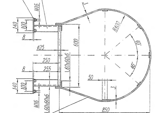
B-B (1:10)
